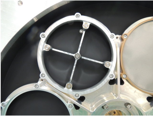
Fig. 18 Picture of the ^{55}\text{Fe} sources ring within the filter wheel disk, with the mounted radioactive sources. The sources are located on the end of the “cross” structure and in the center of the cross. Ring inner diameter is about 9 cm.
