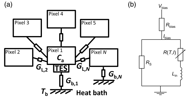
Fig. 1 (a) Thermal model of a multiabsorber TES consisting of N x-ray absorbers of heat capacity C_a , connected to a single TES via a conductance G_{L,i} . The TES and absorbers are weakly thermally coupled to a heat bath of temperature T_b via conductance G_{b,i} (for clarity G_{b,i} is only shown for pixel 1 and pixel N ). (b) Electrical bias circuit for the TES of resistance R(T, I) .
