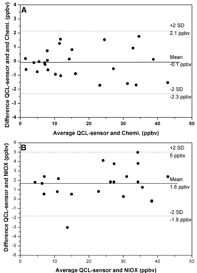
Fig. 7 Bland-Altman plot comparing the QCL-based sensor with chemiluminescence device (a) and with NIOX MINO (b), respectively. (a) Solid line represents the mean difference between values obtained using the QCL-based sensor and chemiluminescence ( -0.1 ppbv). Dashed lines represent the limits of agreement, -2.3 ppbv and 2.1 ppbv. The plot suggests the two sensors are in good agreement. (b) Solid line represents the mean difference between values obtained using the QCL-based sensor and NIOX MINO (1.6 ppbv). Dashed lines represent the limits of agreement, -1.8 ppbv and 5 ppbv; SD is standard deviation. The plot suggests the QCL-sensor and NIOX MINO are quite similar and reveals one outlier.
