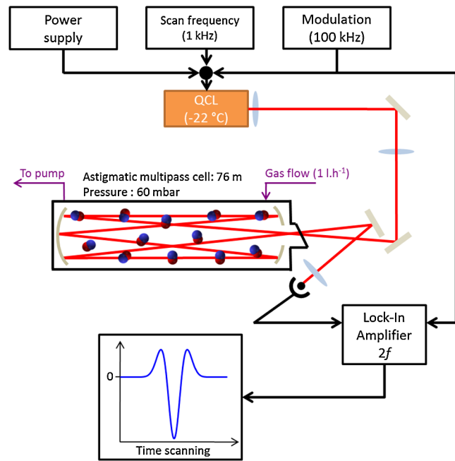
Fig. 1 Schematic of the QCL-sensor. The QCL beam at 5.2 \mu\text{m} is sent into a 30-cm multi-pass cell, thus enhancing the absorption path length to 76 m. Wavelength modulation is performed by modulating the laser current at 100 kHz, and a 2f lock-in amplifier is used to demodulate the signal. (Color online only.)
