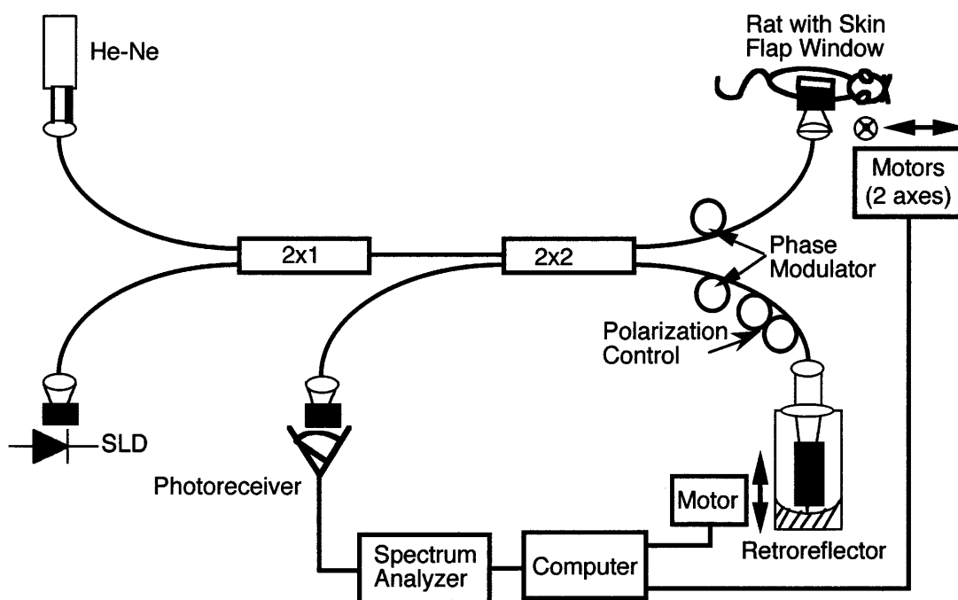
Fig. 2 Optical low-coherence reflectometry system. The SLD has a center wavelength of 855 nm with 300 \mu W power on tissue.
