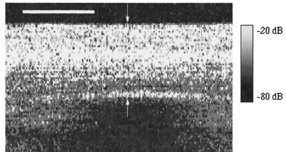
Fig. 9 Cross-section OLCR image of the window model. Arrows denote position of thickness measurement of 520 \mu\text{m} . Bar=500 \mu\text{m} .
