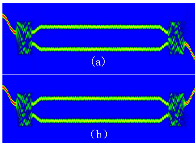
Fig. 3 Optical field distribution calculated using 3-D-BPM: (a) cross state when no power is applied on the switch and (b) bar state when the switch is driven by appropriate power.
