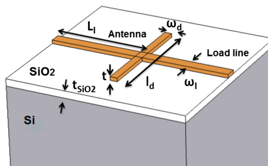
Fig. 1 Spatial dimensions of dipole antenna.
