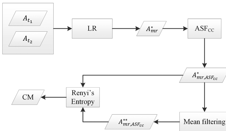
Fig. 3 Change detection flowchart. A_{t_1} , A_{t_2} : input amplitude image pair; LR: log-ratio calculation; A_{mr}^* : maximum ratio image; ASF_{CC} : connected alternating sequential filtering; A_{mr,ASF_{CC}}^* : denoised maximum ratio image; mean filtering: usage of a mean 3 \times 3 box filter; A_{mr,ASF_{CC}}^{**} : mean-filtered denoised maximum ratio image; Rényi's entropy: application of Rényi's unsupervised threshold calculation; CM: binary change map.
