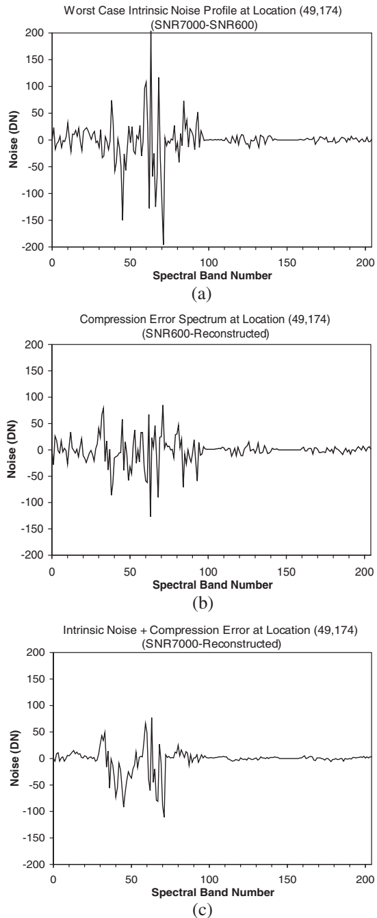
Figure 5.8 Profiles of (a) the worst-case intrinsic noise of the original data at location (49, 174), (b) compression error introduced by SAMVQ at a compression ratio of 20:1, and (c) overall noise (i.e., intrinsic noise with compression error) at the same location (reprinted from Ref. 1).
