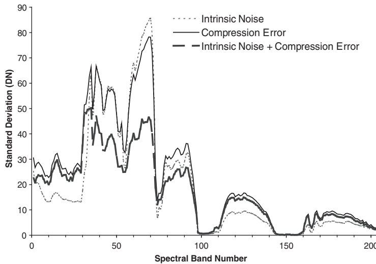
Figure 5.11 Standard deviations of single-band images for intrinsic noise, compression error (using HSOCVQ at a compression ratio 10:1), and overall noise (i.e., intrinsic noise with compression error). Reprinted from Ref. 1.
