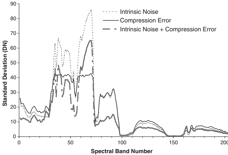
Figure 5.10 Standard deviations of single-band images for intrinsic noise, compression error (using SAMVQ at a compression ratio 20:1), and overall noise (intrinsic noise with compression error). Reprinted from Ref. 1.
