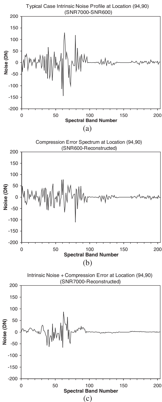
Figure 5.9 Profiles of (a) intrinsic noise of the original data of a randomly selected ground-sample pixel (94, 90), (b) compression error introduced by SAMVQ at a compression ratio of 20:1, and (c) overall noise (i.e., intrinsic noise with compression error) at the same location (reprinted from Ref. 1).
